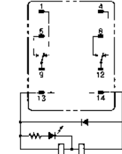
MY2N1-D2/MY2IN1-D2 (DC Models Only)
