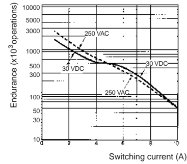
MY2 (Resistive Loads)
