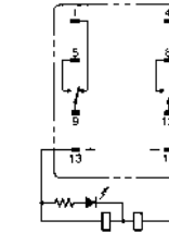
MY2N1/MY2IN1 (DC Models Only)
