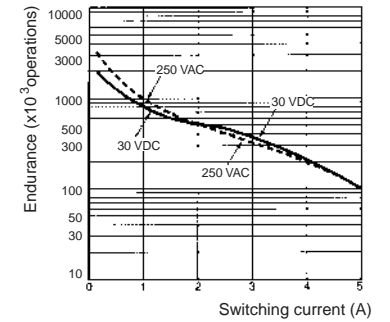
MY2 (Inductive Loads)
