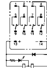
MY4(Z)N1-D2/MY4(Z)IN1-D2 (DC Models Only)
