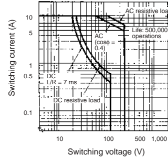
LY3 and LY4 Maximum Switching Power
