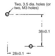
Mounting holes
