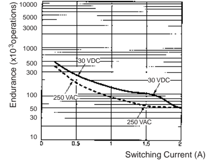
MY4Z (Inductive Loads)
