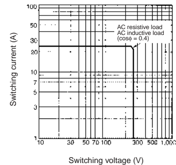
G7L-2A-T/G7L-2A-B Maximum Switching Power
