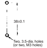
Mounting holes
