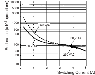
MY4Z (Resistive Loads)
