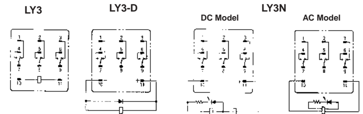
Terminal Arrangement/Internal Connections (Bottom View)
