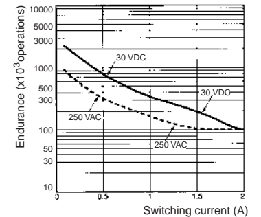
MY4 (Inductive Loads)
