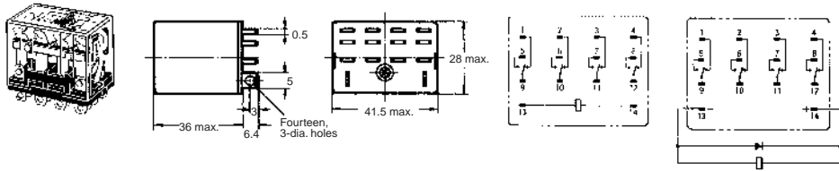
Terminal Arrangement/Internal Connections (Bottom View)
