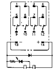
MY4(Z)N-D/MY4(Z)IN-D2 (DC Models Only)
