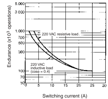
Endurance
