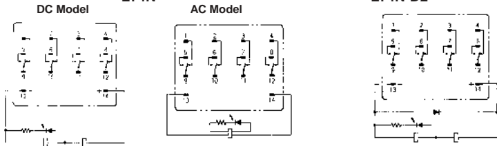
Terminal Arrangement/Internal Connections (Bottom View)
