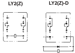
Terminal Arrangement/Internal Connections (Bottom View)
