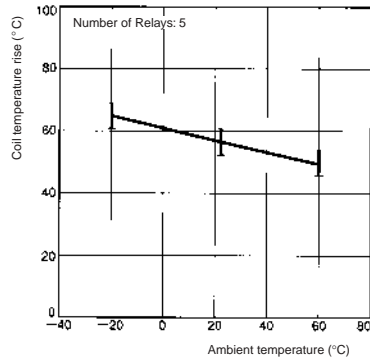
G7J-4A 24 VDC
