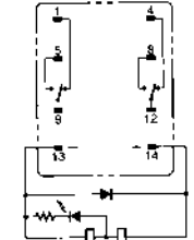
MY2N-D2/MY2IN-D2 (DC Models Only)
