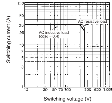
G7L-1A-T/G7L-1A-B Maximum Switching Power
