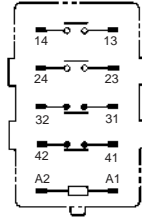
G7J-2A2B-P(B) (T)
