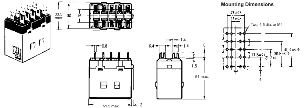
G7J-4A-P, G7J-4A-PZ, G7J-3A1B-P, G7J-3A1B-PZ, G7J-2A2B-P
