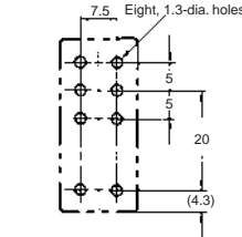
Terminal Arrangement (Bottom View)
