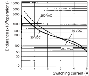
MY4 (Resistive Loads)
