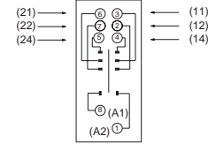
Terminal Arrangement (Top View)
