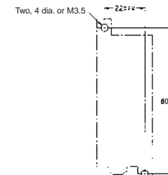
Mounting Hole Placement Diagram (Top View)
