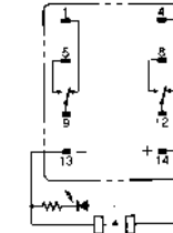
MY2N/MY2IN (DC Models)
