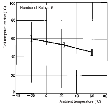
G7J-4A 24 VDC
