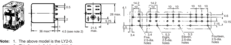
PC Board Holes (Bottom View)
