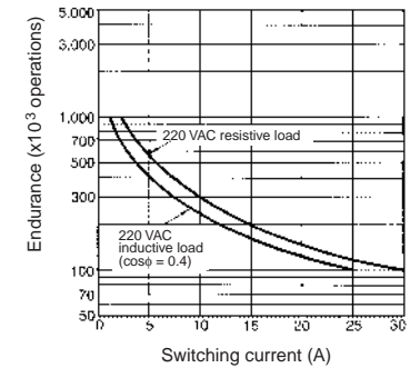
Endurance
