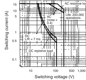
LY2 Maximum Switching Power
