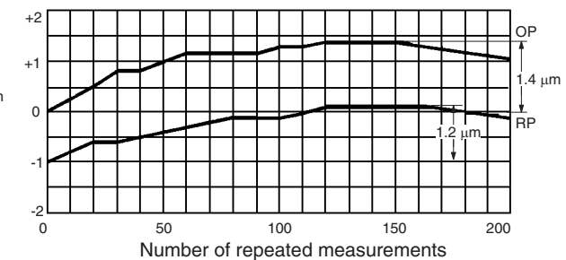
Limit Type (Solid-state Output) With Repeat Accuracy of 3 μm max. D5A-8□□□ Series, D5A-9□□□ Series
